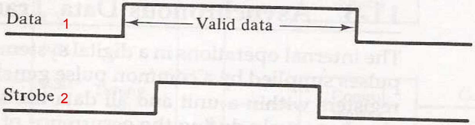
(b) Timing diagram
