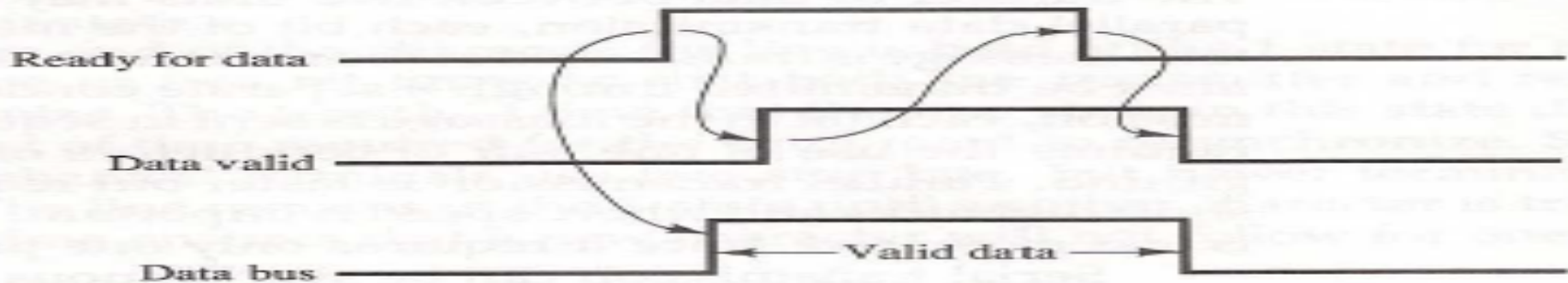
(b) Timing diagram
