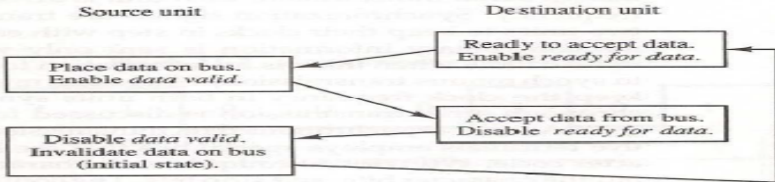
(c) Sequence of events
