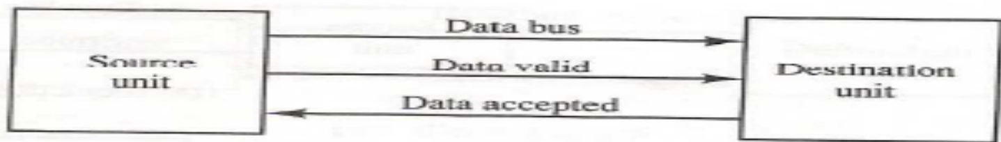
(a) Block diagram
